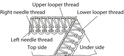
Fig. 5 Right needle thread loose and visible on under side of fabric
