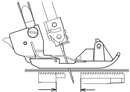
Negative differential feed
