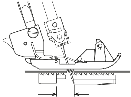
Positive differential feed
