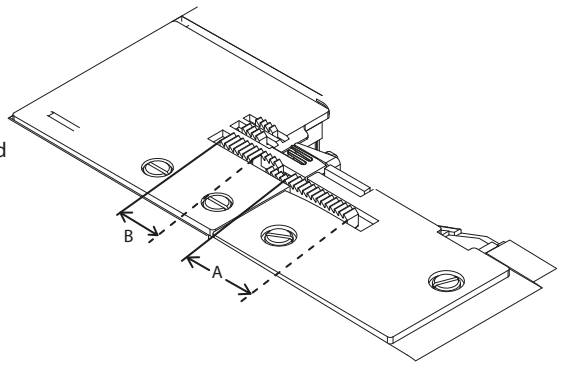
Differential feed dogs
