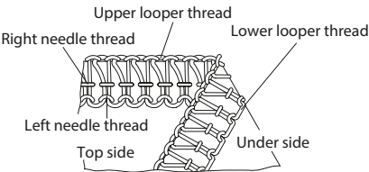
Fig. 4 Left needle thread loose and visible on under side of fabric
