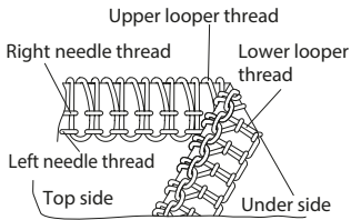
Fig. 2 Upper looper thread pulled to top side
