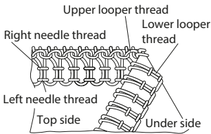
Fig. 3 Lower looper thread pulled to top side
